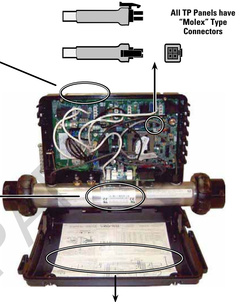
Heater Element Specifications Are Shown on the Heater Tube Label
